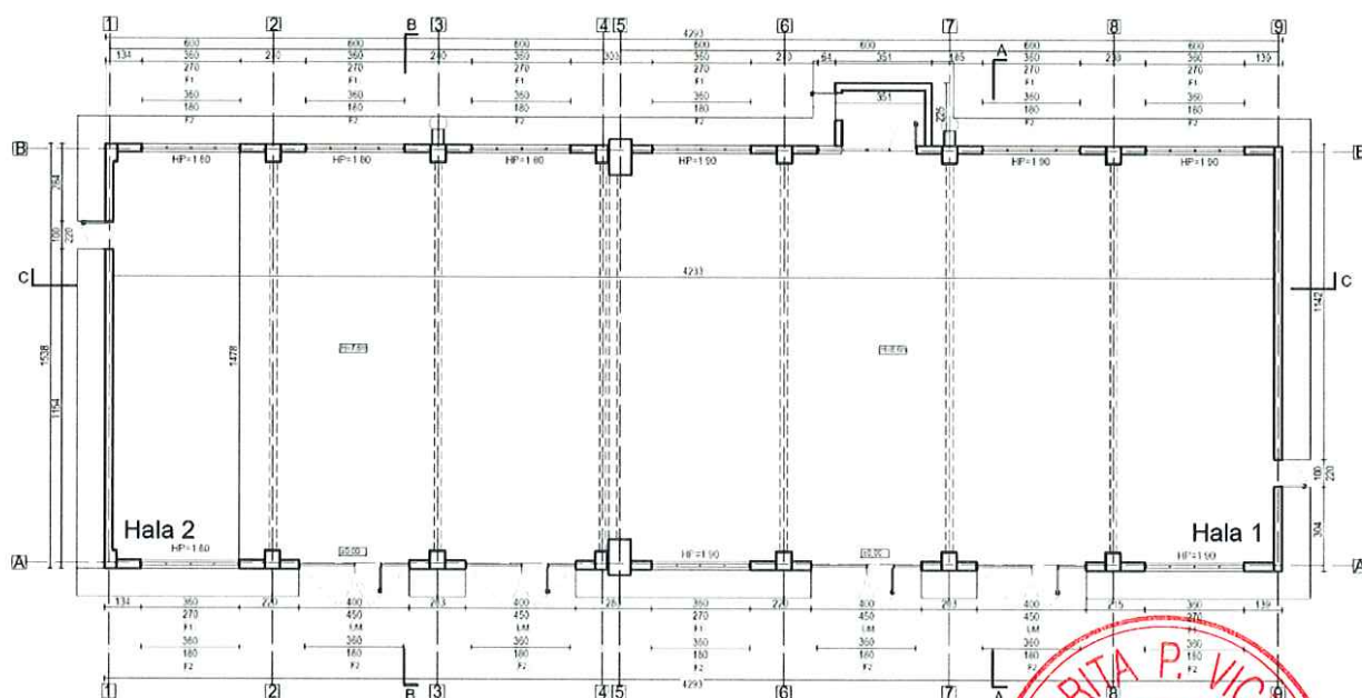
RELEVU PARTER
