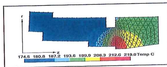
2D-Axisymmetric Finite Element Analysis review showing temperature distribution.
